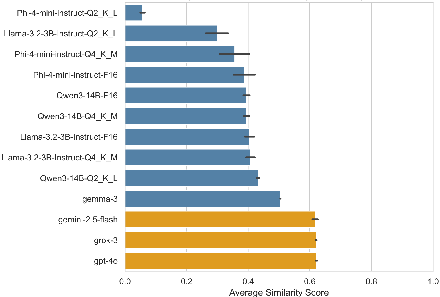
Average WordNet Similarity Score by Model
